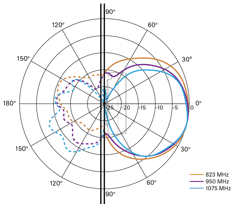
UHF (823-1075 MHz) 垂直 [dB]
