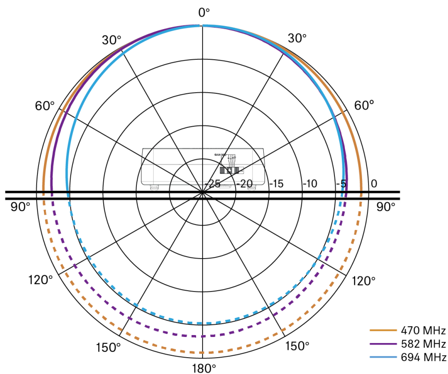
UHF (823-1 075 MHz) vertical [dB]
