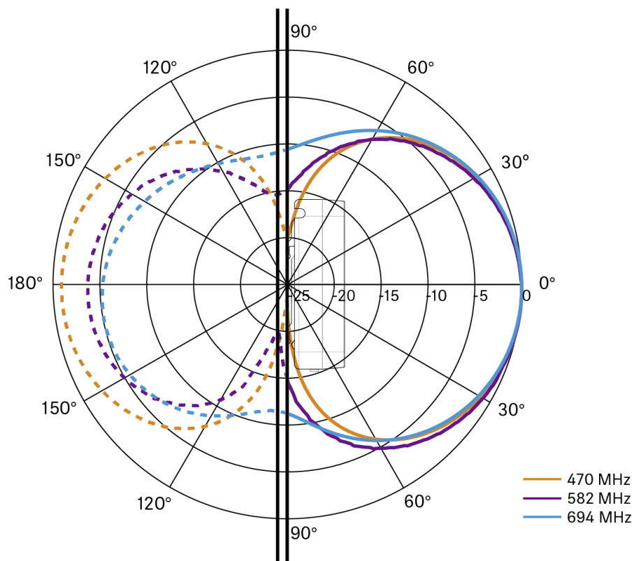
UHF (470-694 MHz) vertical [dB]
