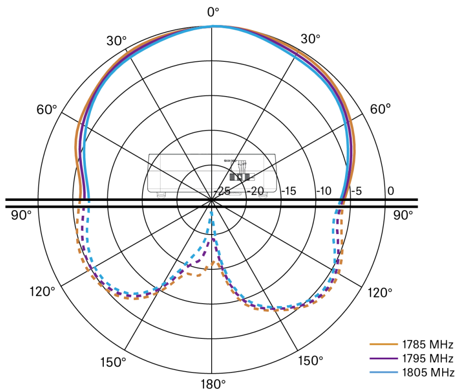
1G8 horizontal [dB]
