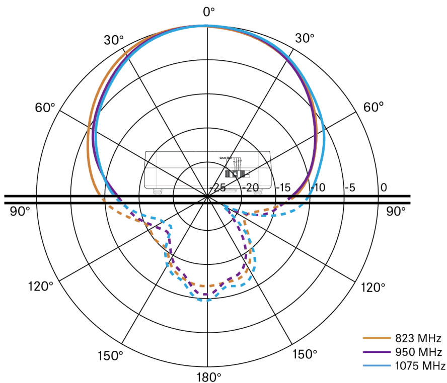
1G8 vertical [dB]
