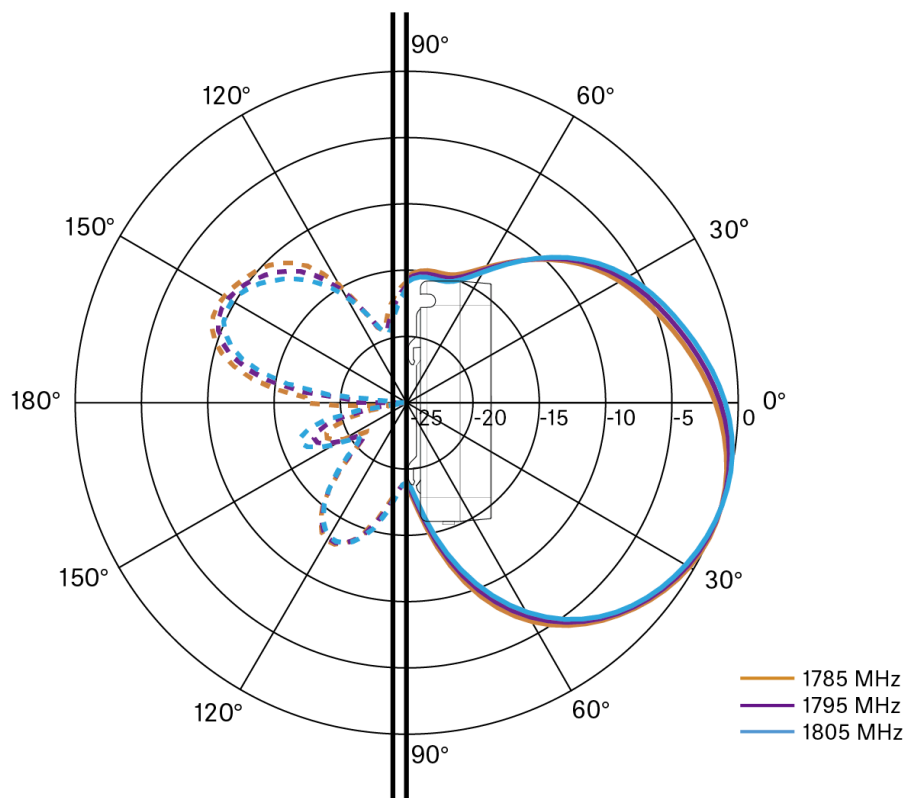
1G8 horizontal [dB]
