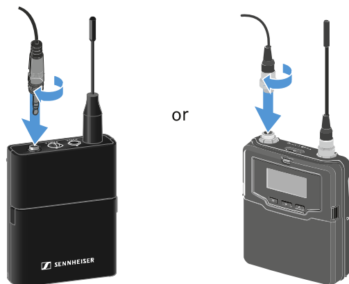
3.5 mm jack plug
