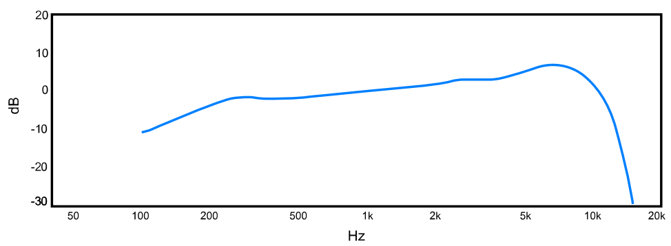
Frequenzgang
