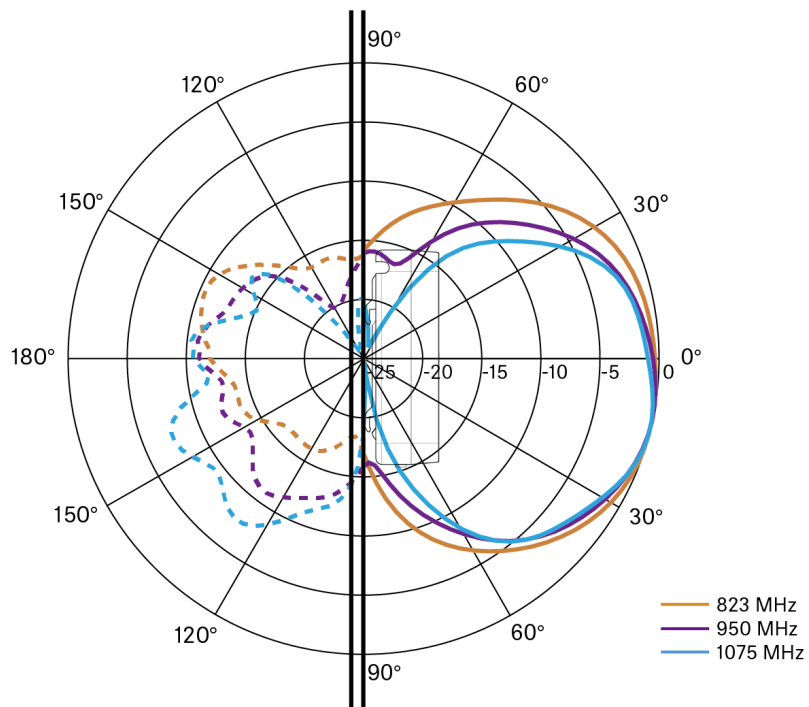
UHF (823-1075 MHz) Vertikal [dB]
