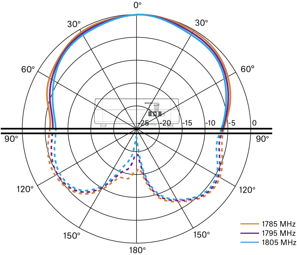
1G8 Horizontal [dB]
