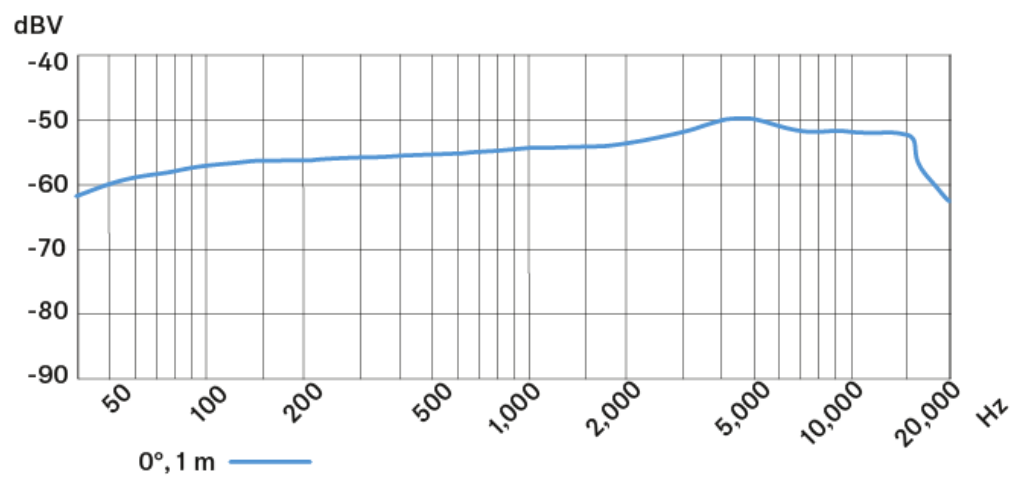
Frequenzgang
