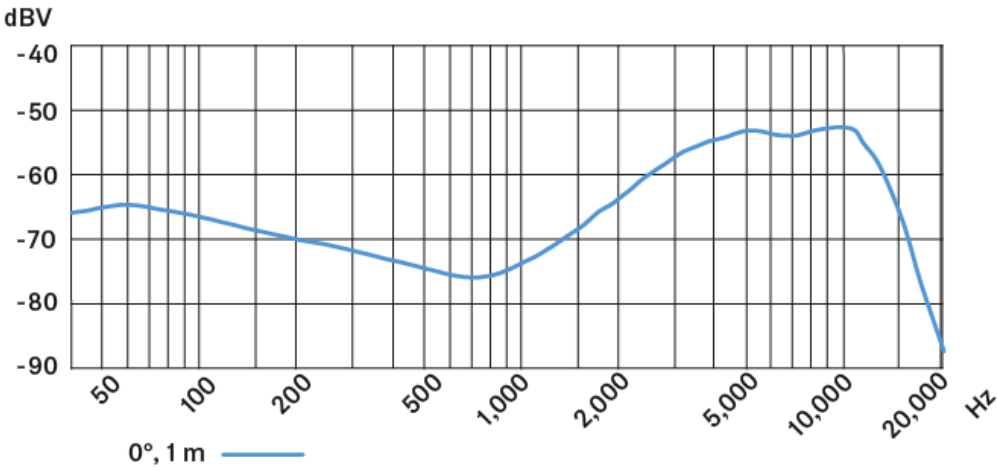
Frequenzgang
