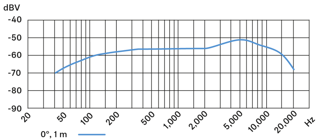
Frequenzgang
