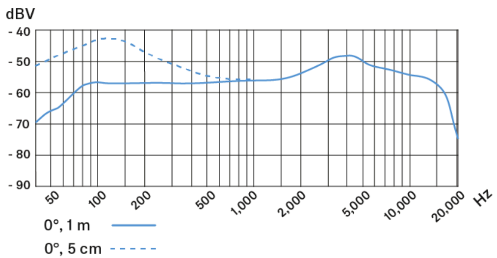
Frequenzgang
