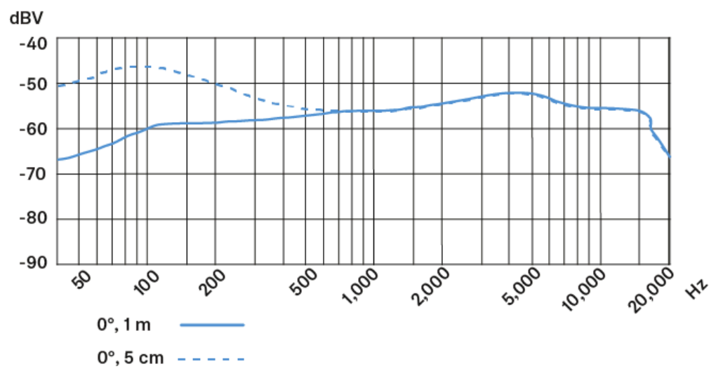
Frequenzgang
