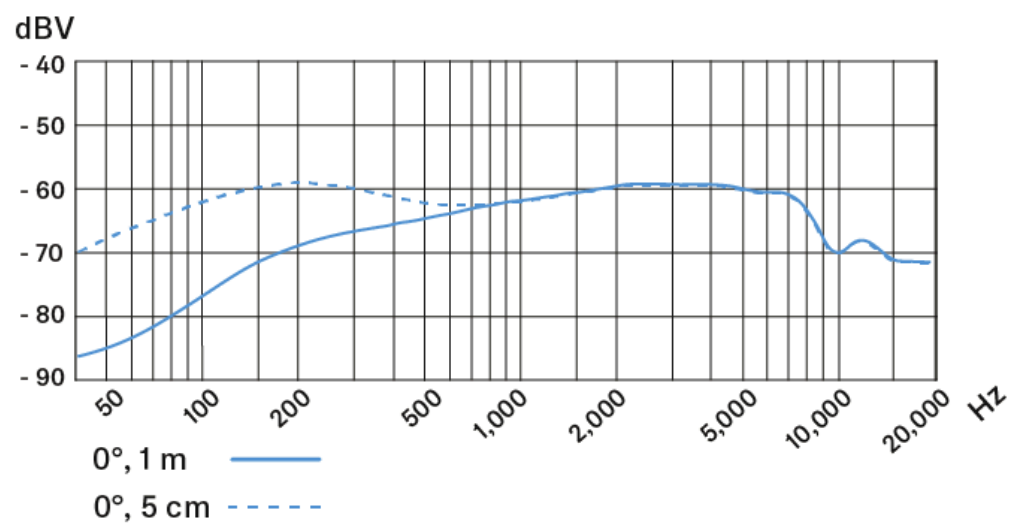
Frequenzgang
